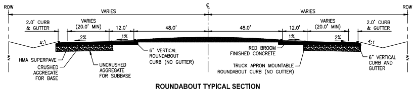
ROUNDABOUT TYPICAL SECTION
