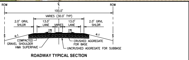
ROADWAY TYPICAL SECTION
